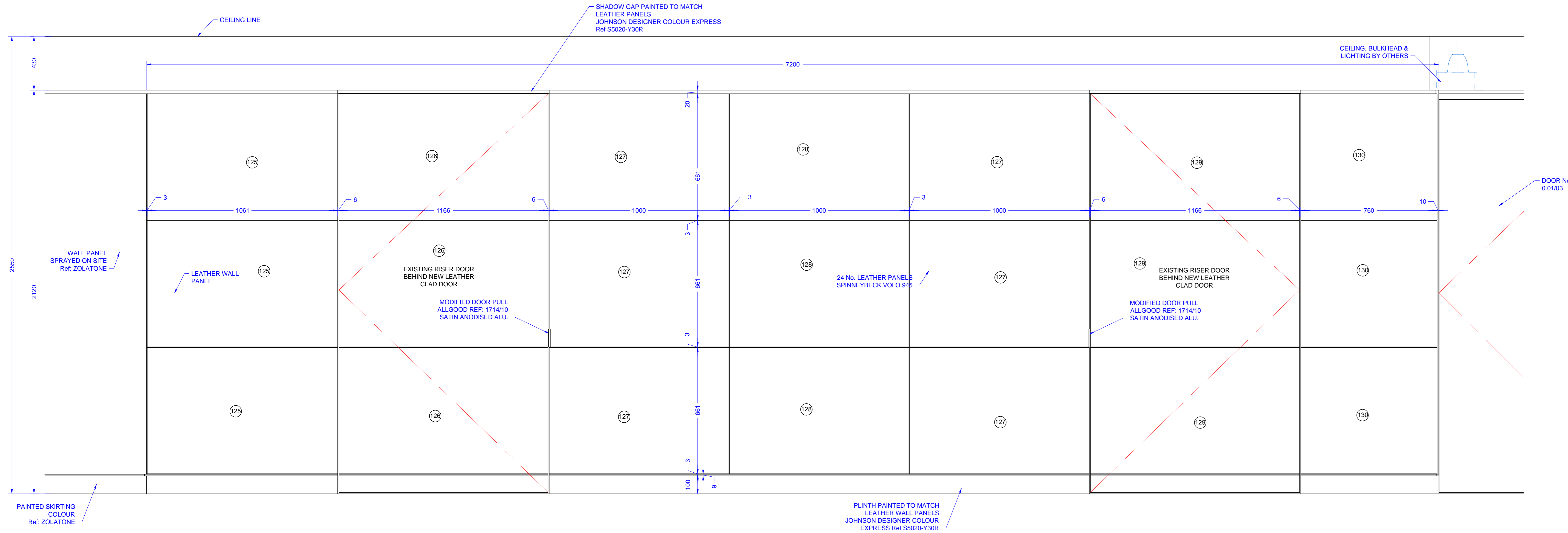
ELEVATION 'A'
