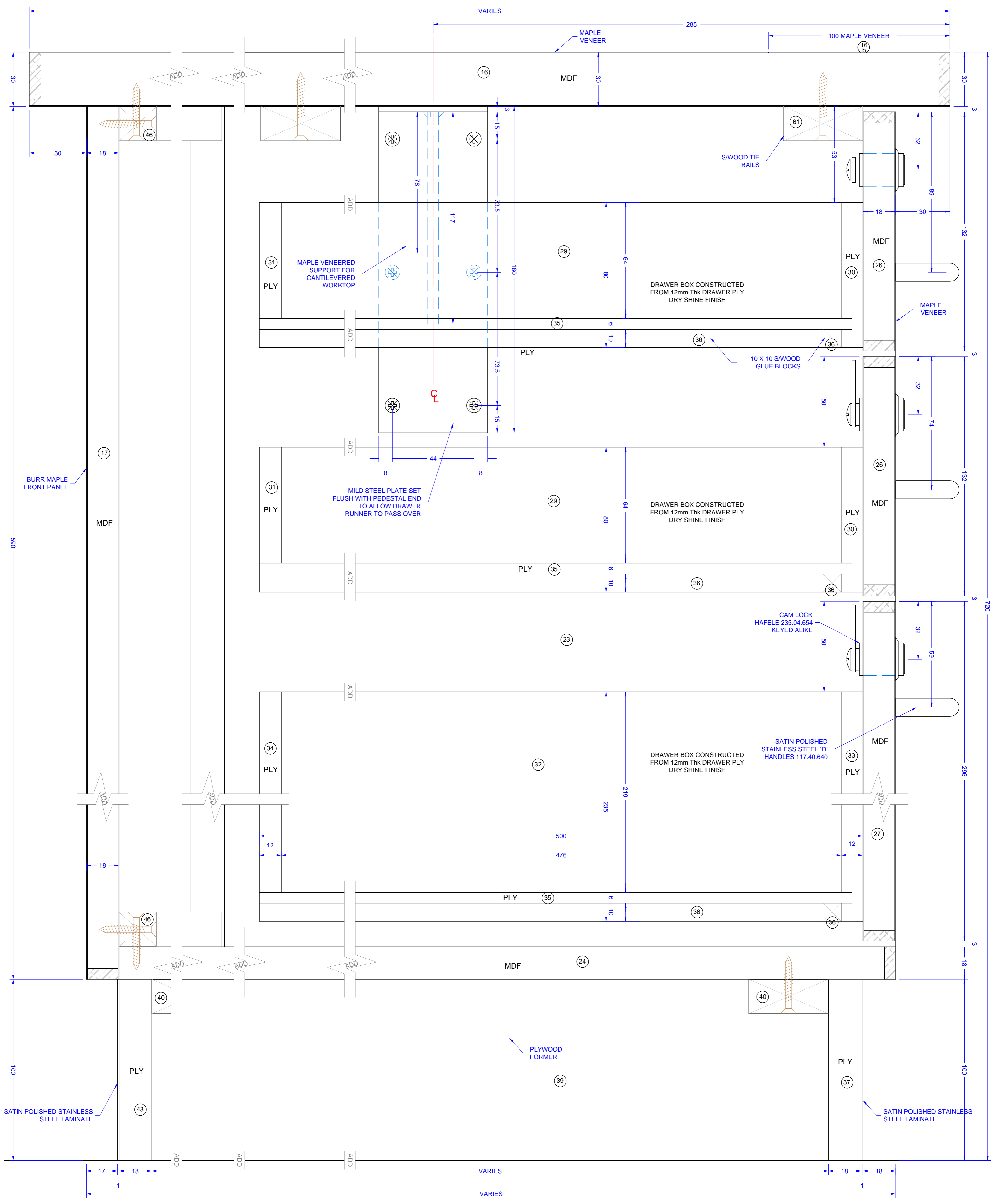
HEIGHT SECTION B-B
